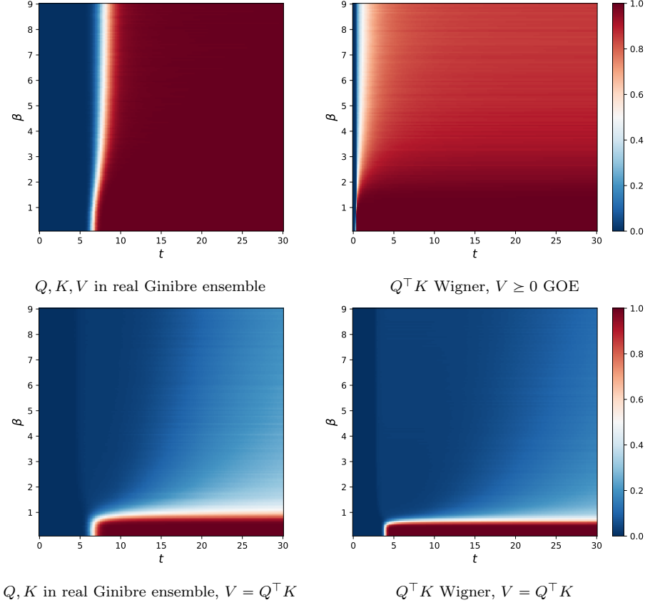
Figure 4. Phase diagrams (see Figure 2 for explanations) for some choices of random matrices (Q, K, V) ; here d = 128, n = 32 . Sharp phase transitions as well as metastable regions appear in all cases.
